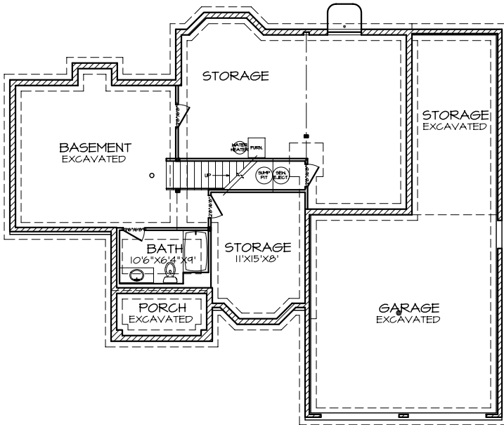
1 FOUNDATION PLAN A-3
