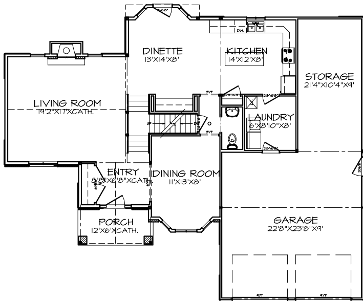
1 FIRST FLOOR PLAN A-4
